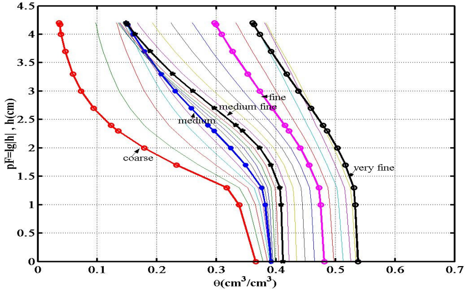
Fig. 2. Correlations between pF and \theta , for Subsoils.
