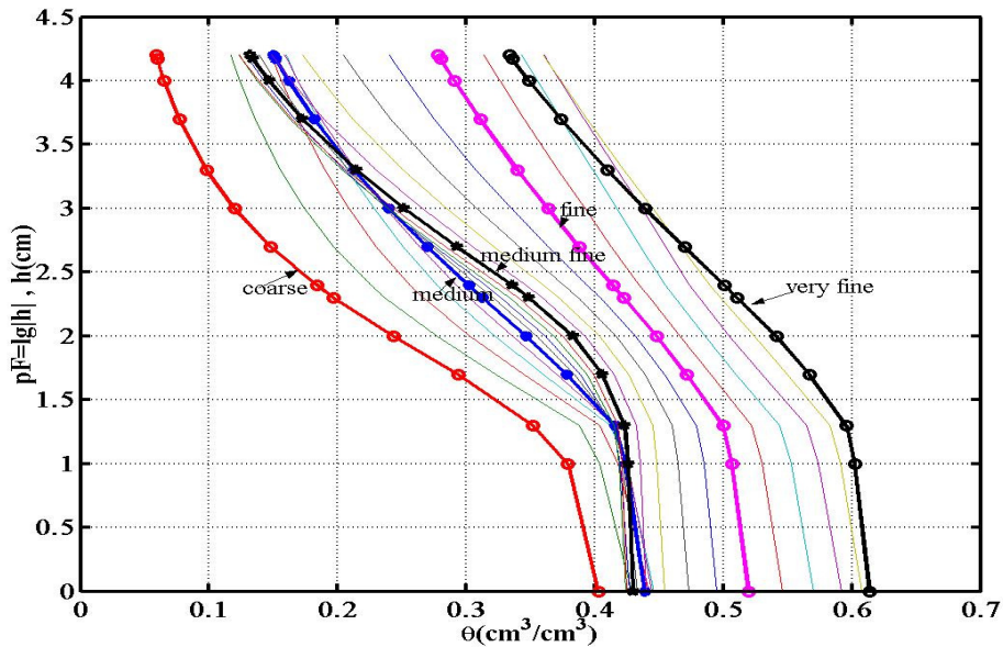
Fig. 1. Correlations between pF and \theta , for Topsoils.
