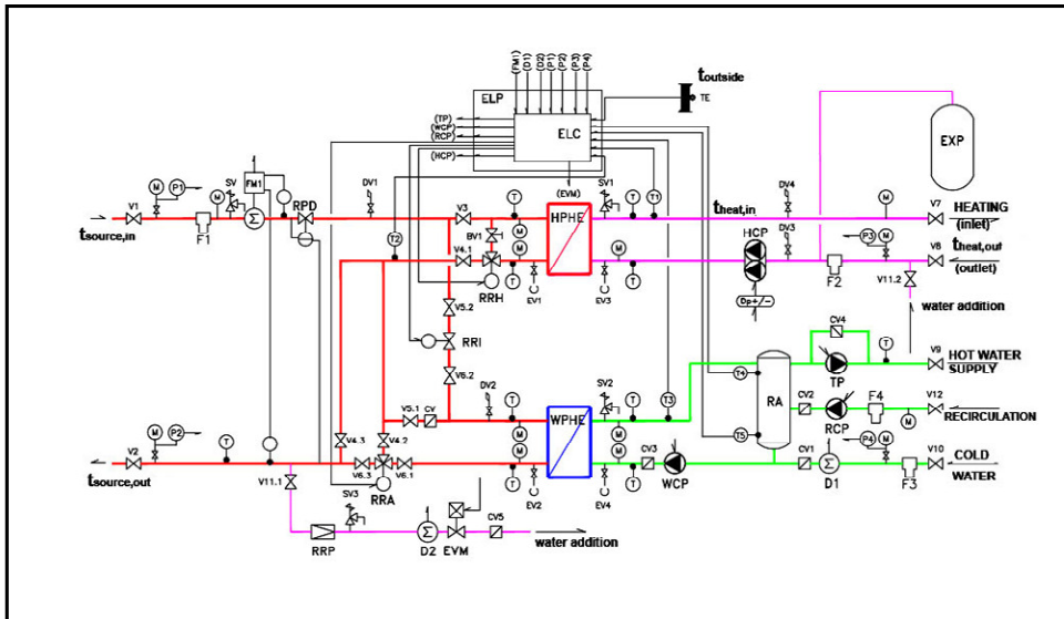
Fig.1: Detailed operation scheme of the small-scale substation
